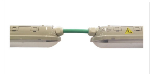
CONNECTION OF FEW LUMINAIRES BETWEEN EACH OTHER 1563610L002 INC.ELEC LC EST/ONIX
